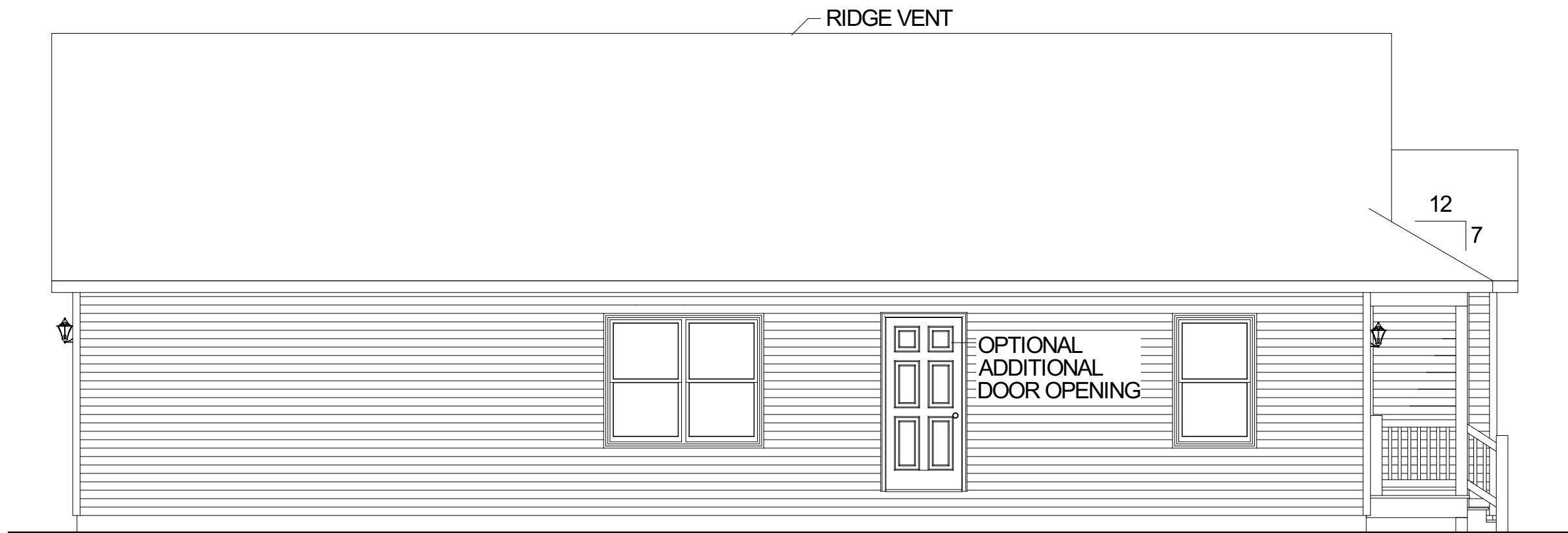
ACCESS TO GRADE ON-SITE BY OTHERS LEFT ELEVATION
