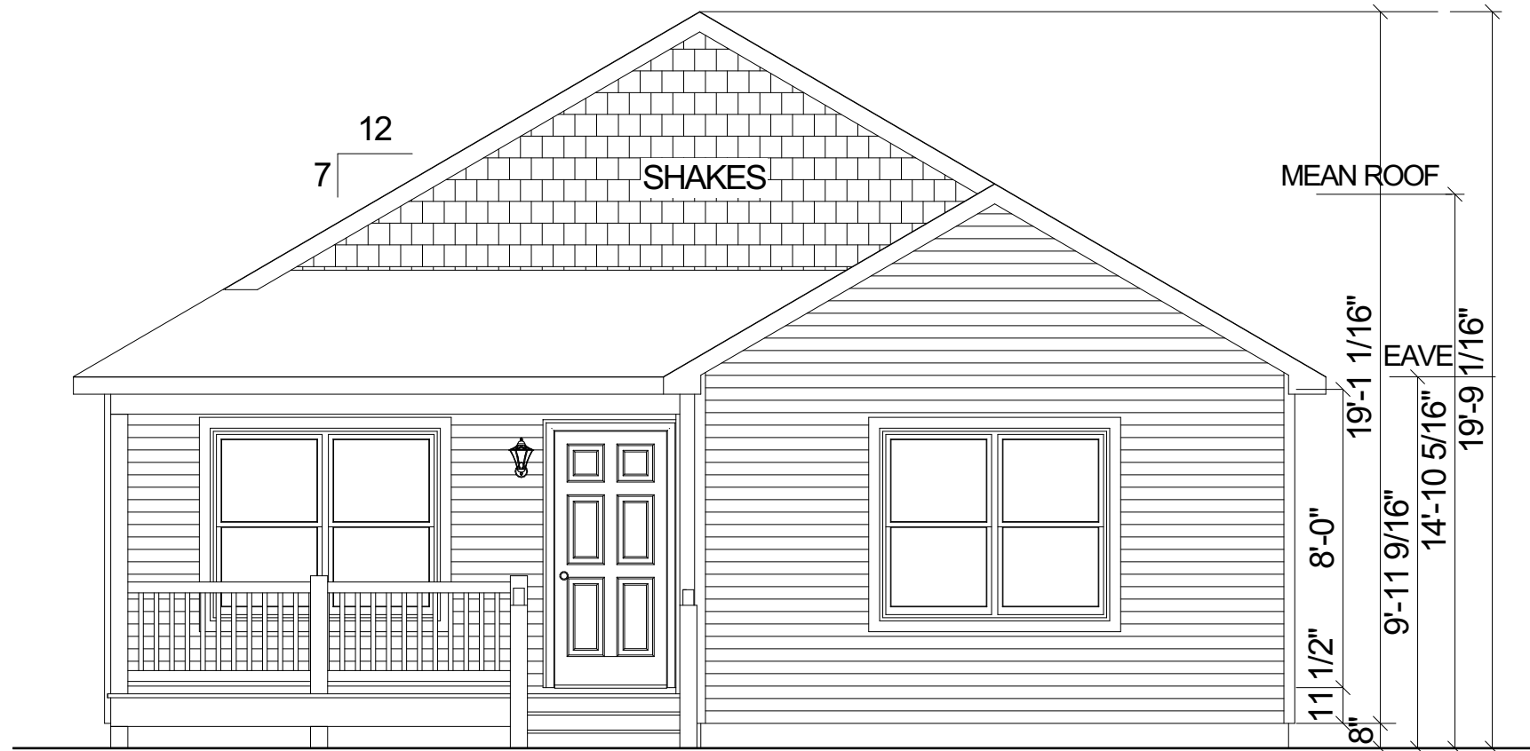
FRONT ELEVATION
