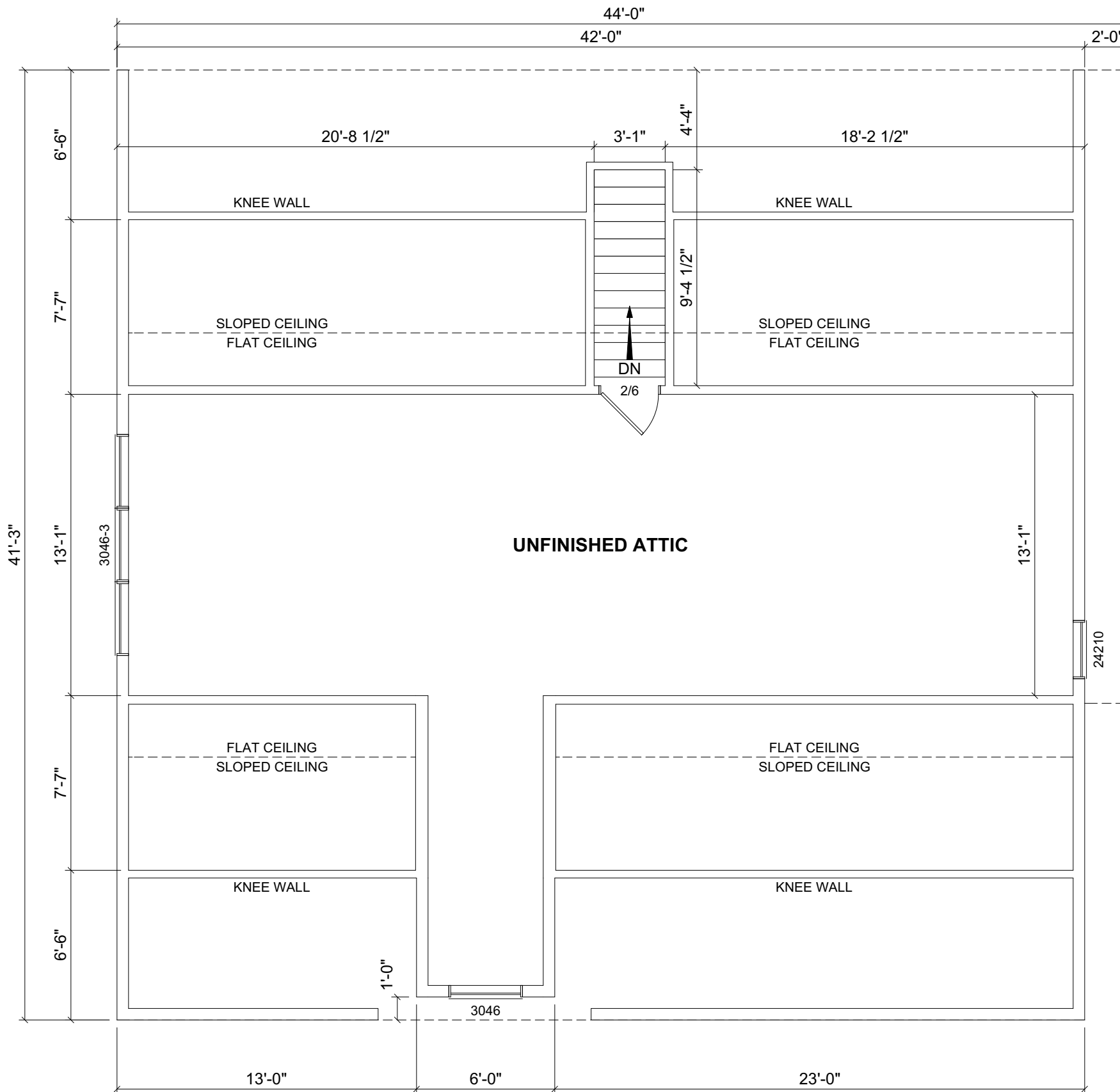
PROPOSED 2ND FLOOR PLAN THE ATTIC IS NOT FINAL UNTIL TRUSS DESIGNED, INTERIOR MATERIALS SUPPLIED & INSTALLED ON-SITE BY OTHERS.
