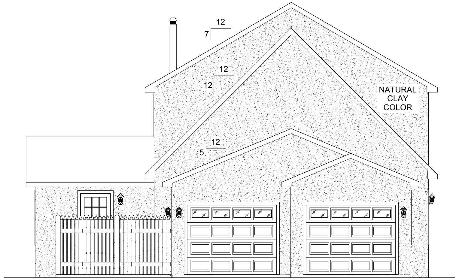
LEFT ELEVATION
