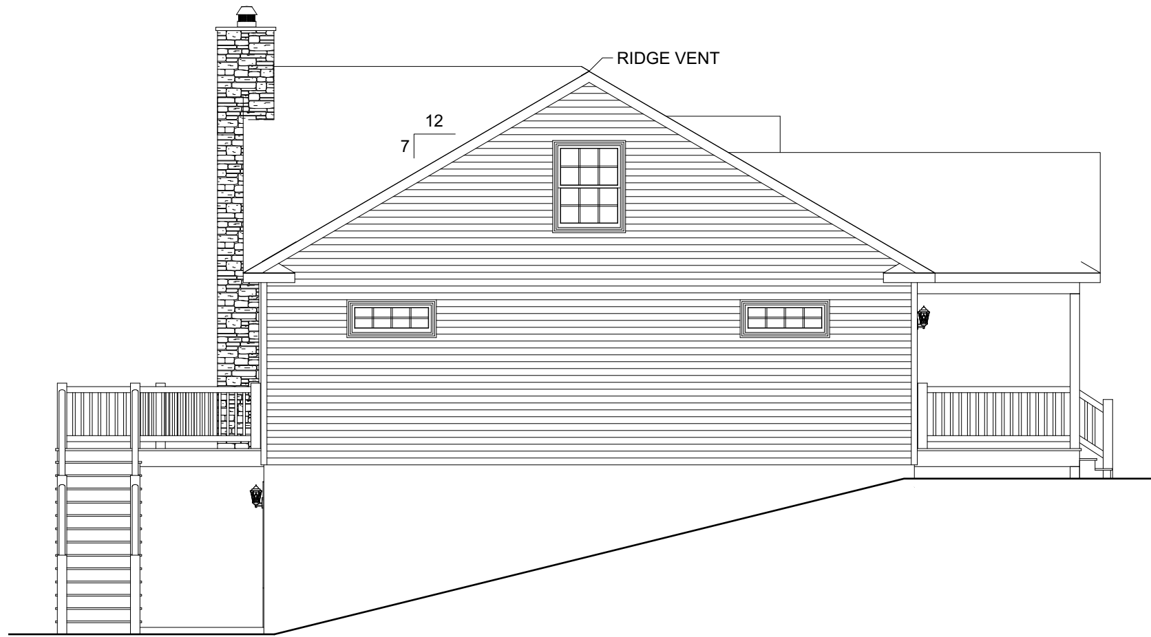
LEFT ELEVATION
