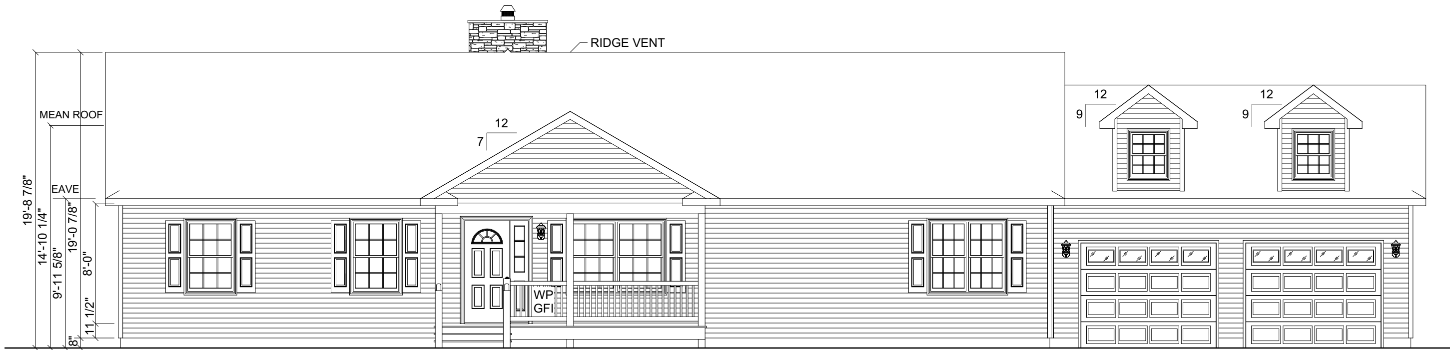
FRONT ELEVATION
