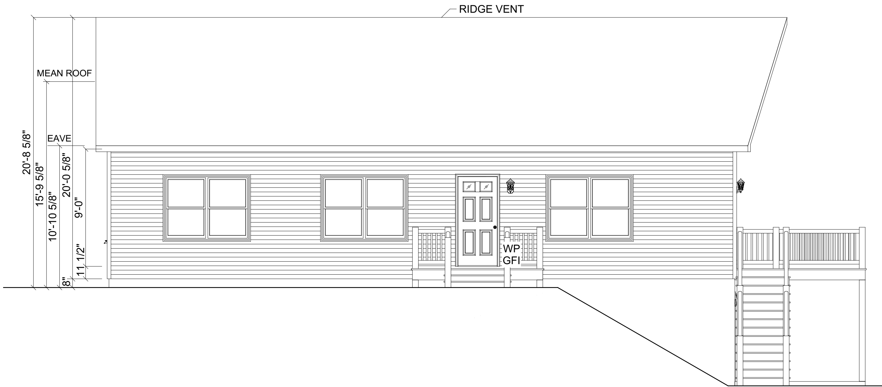
FRONT ELEVATION
