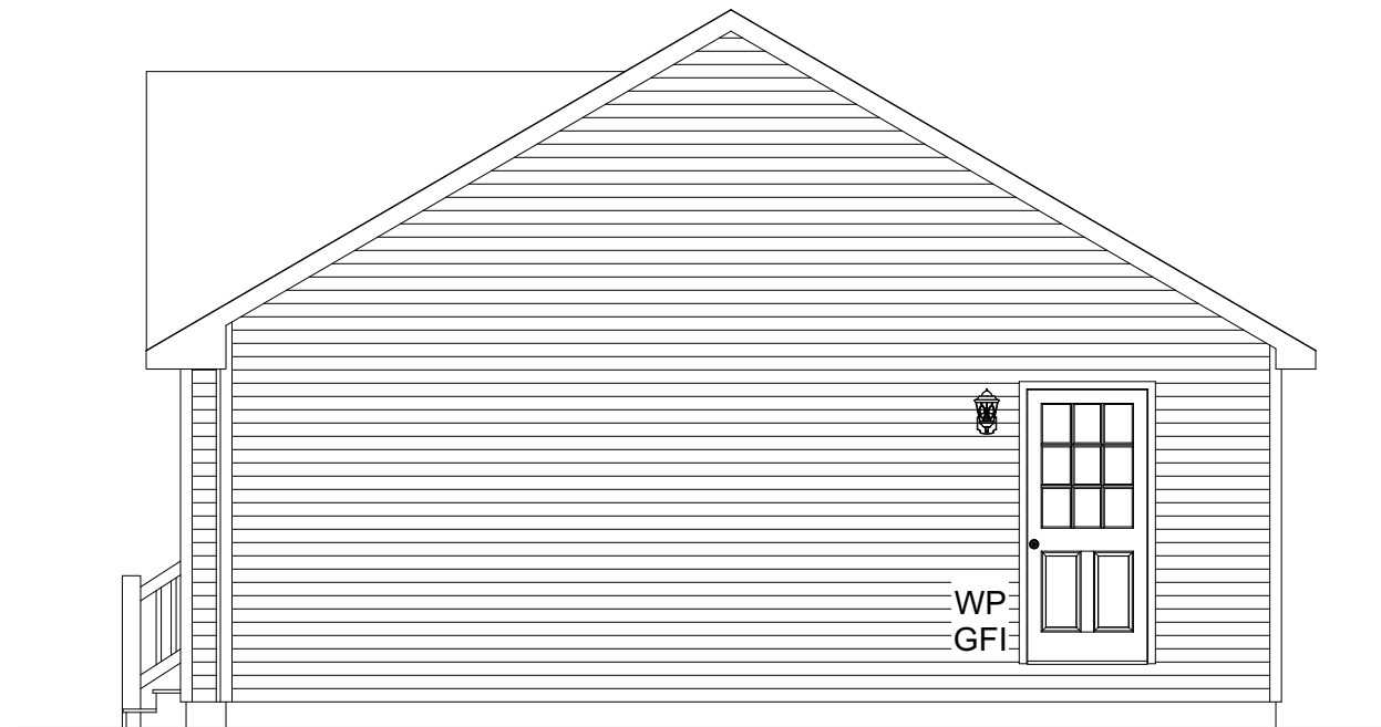
LEFT ELEVATION
