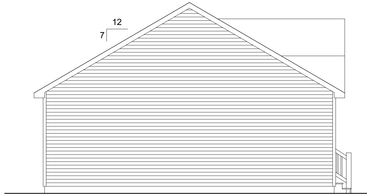
LEFT ELEVATION
