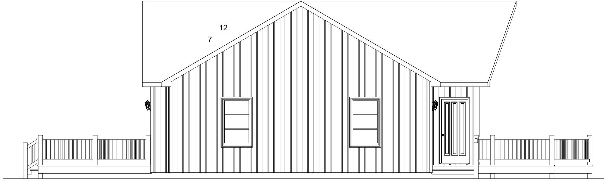
LEFT ELEVATION
