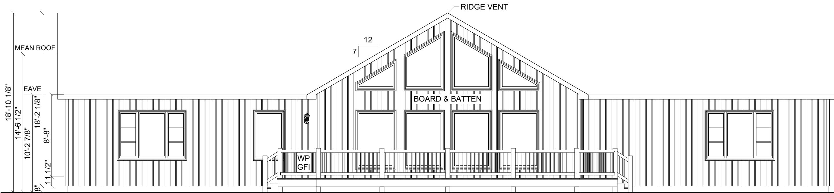
FRONT ELEVATION
