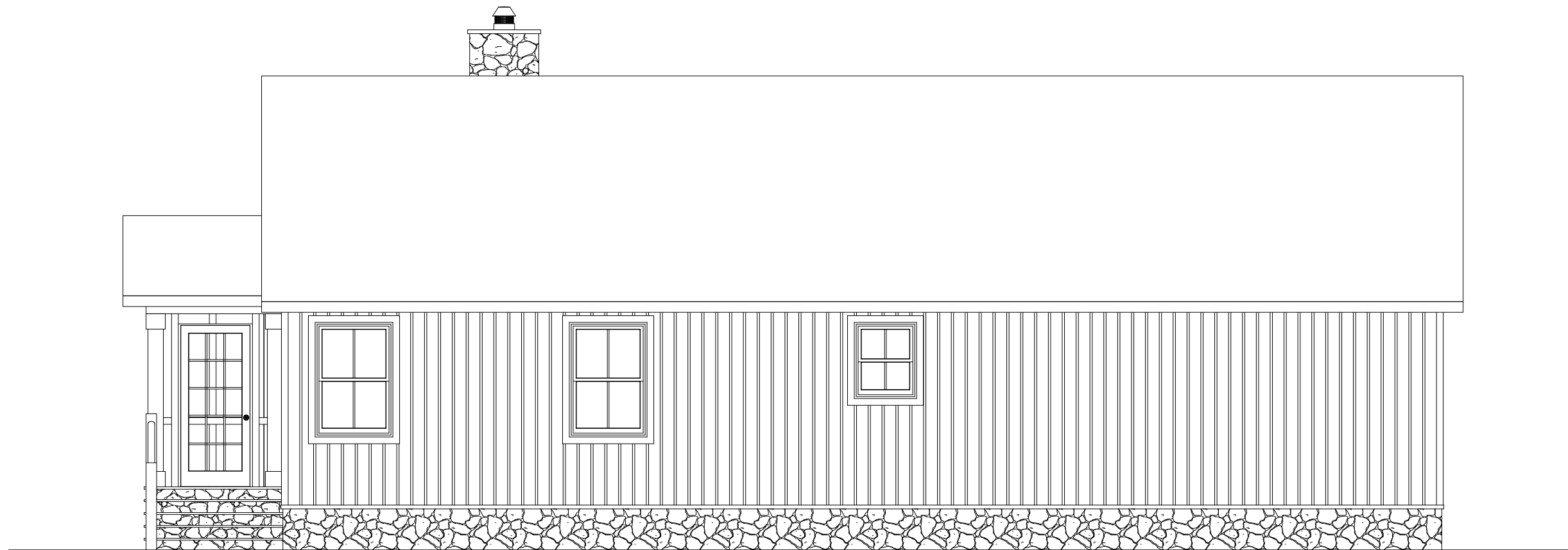
REAR ELEVATION
