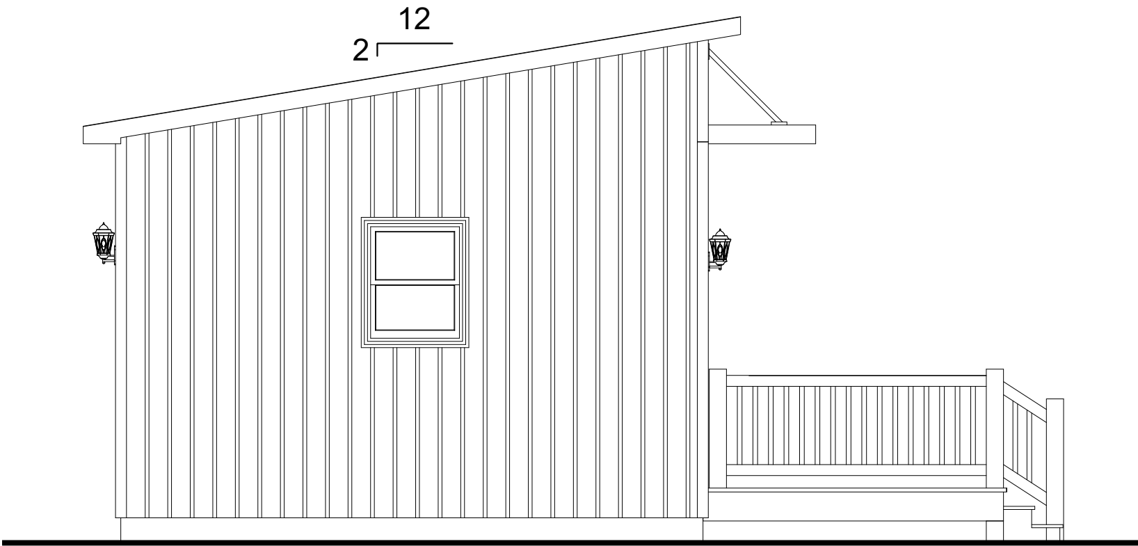
LEFT ELEVATION
