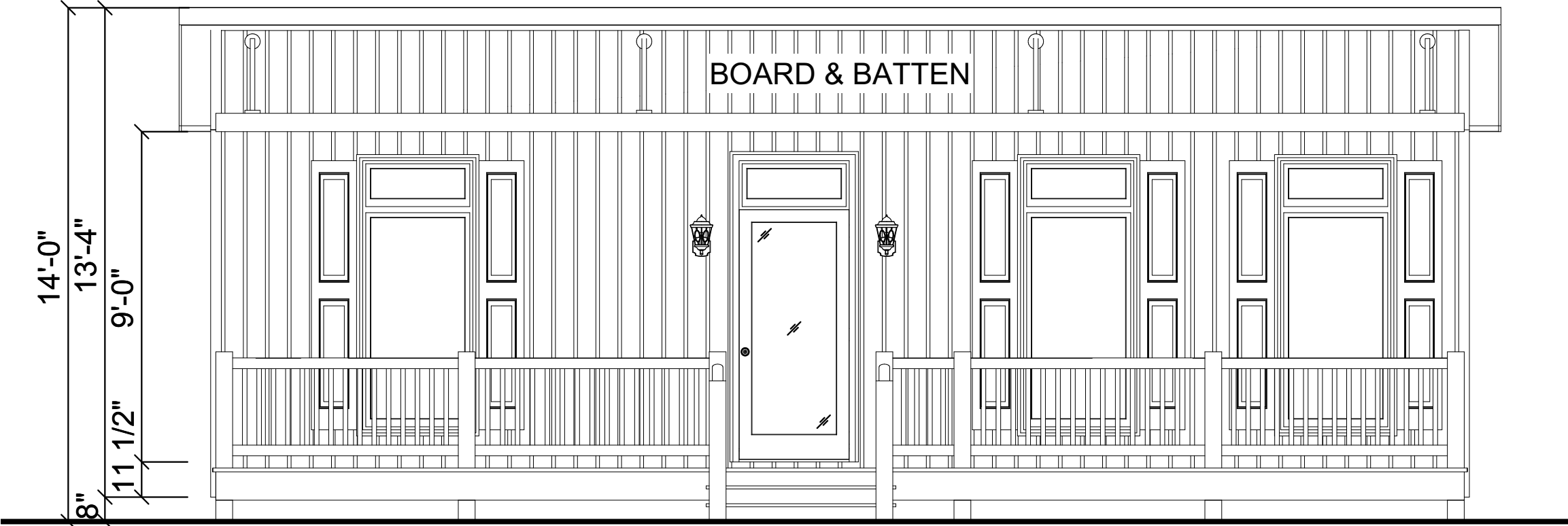
FRONT ELEVATION
