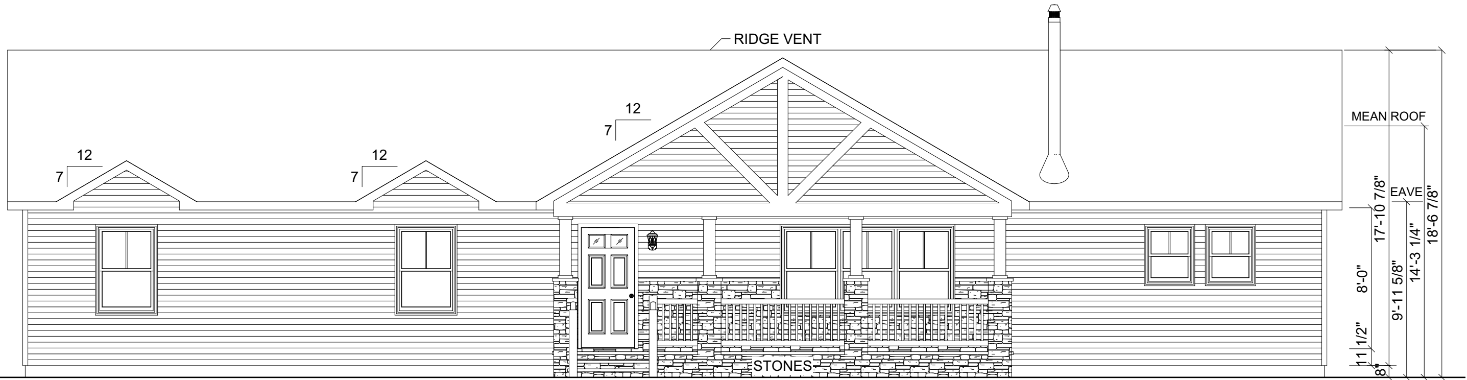
FRONT ELEVATION
